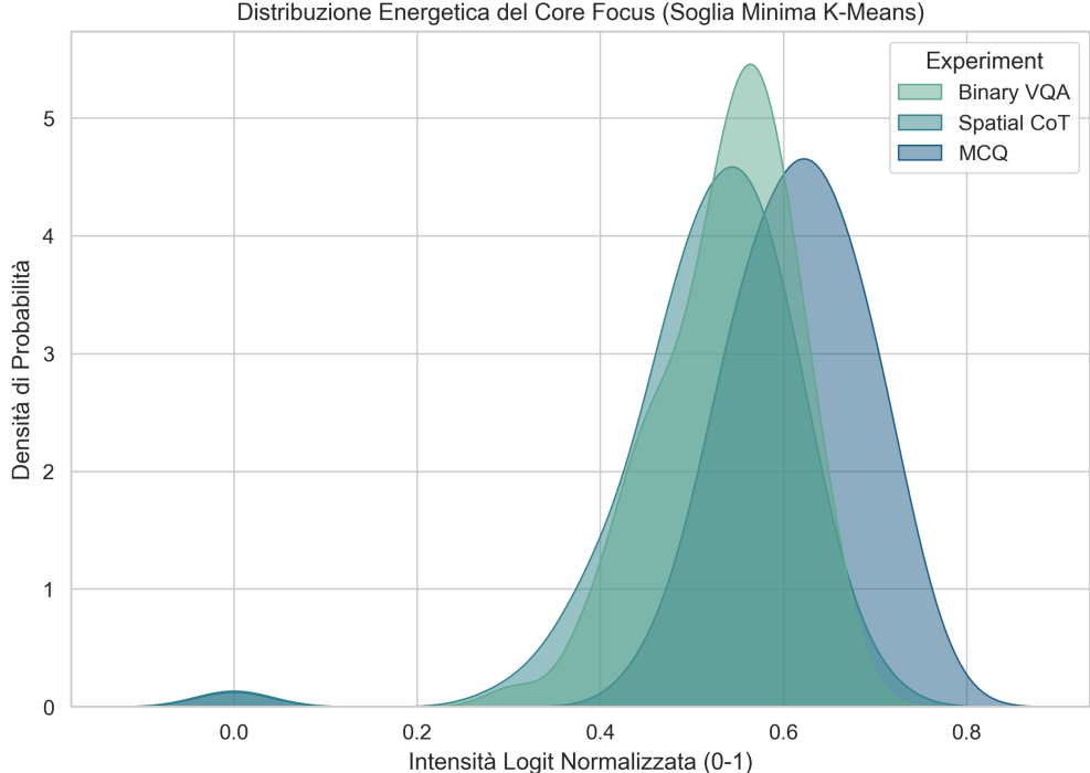
Figure 6: Probability density of the normalized Logit intensity within the Core Focus (K-Means Threshold).
