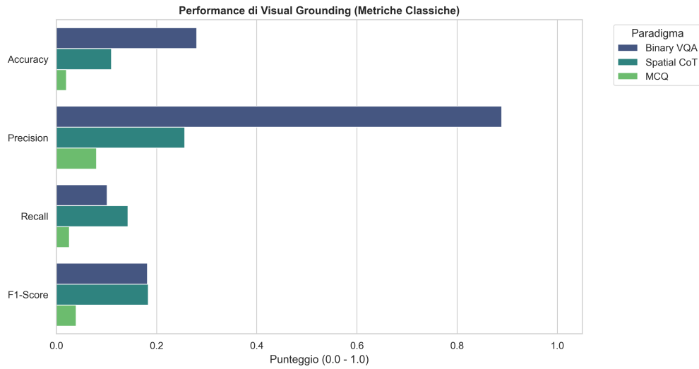
Figure 4: Comparison of classical evaluation metrics (Accuracy, Precision, Recall, F1-Score) strictly based on visual grounding.
