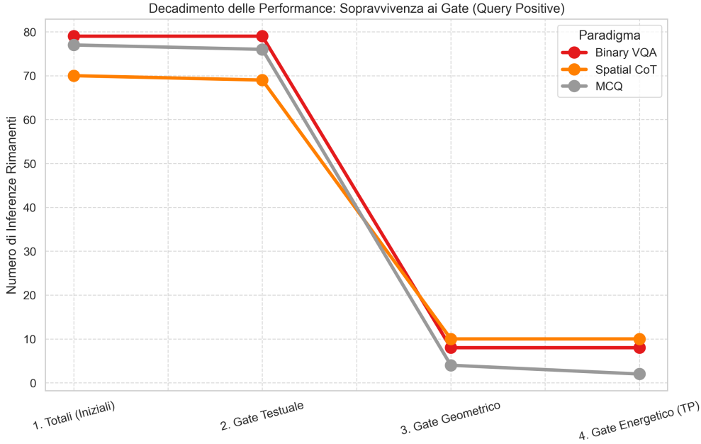
Figure 1: Performance decay (Gate Survival Rate) for positive queries across the 4-Gate validation pipeline.
