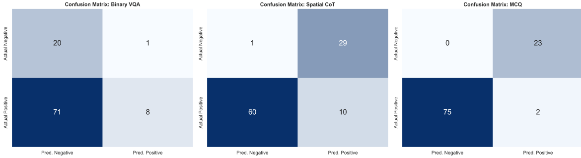
Figure 3: Confusion Matrices calculated using Strict Visual Grounding criteria.
