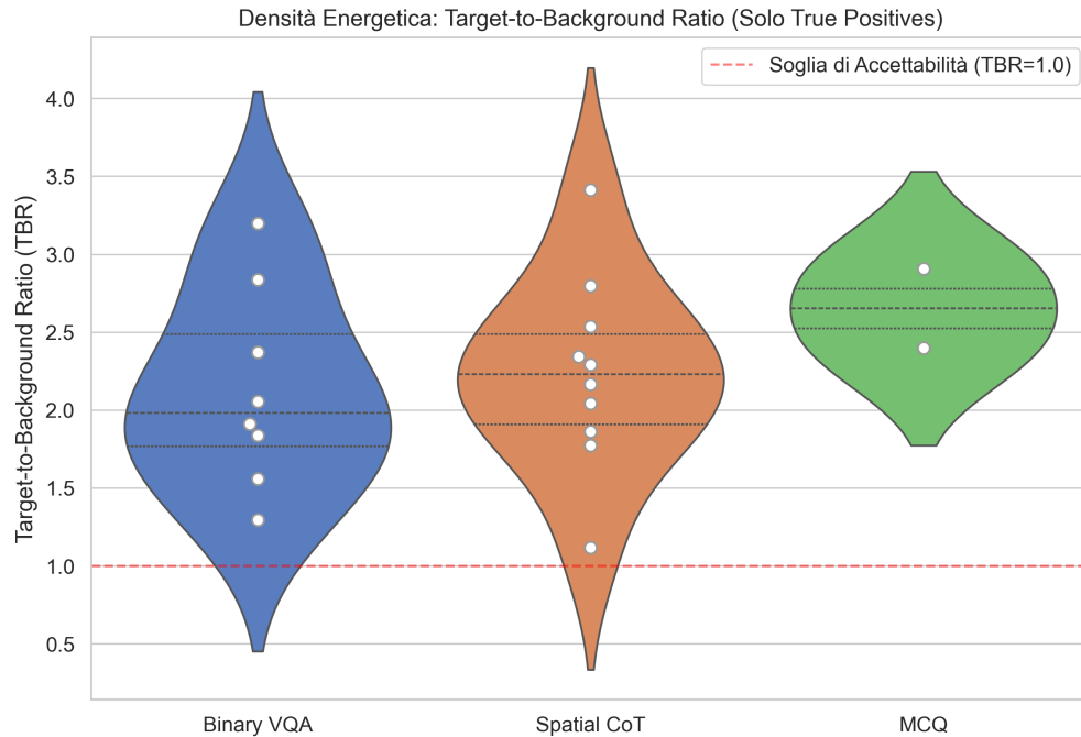
Figure 5: Density distribution of visual confidence (Target-to-Background Ratio) for verified True Positives.
