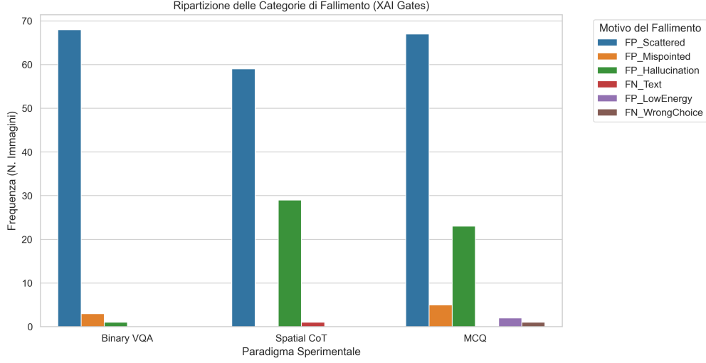
Figure 2: Distribution of specific failure categories across the XAI validation gates.
